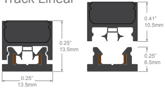
Track Linear
