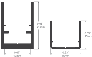
Aluminium Housing
