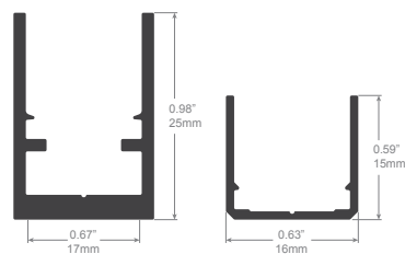
Aluminium Housing
