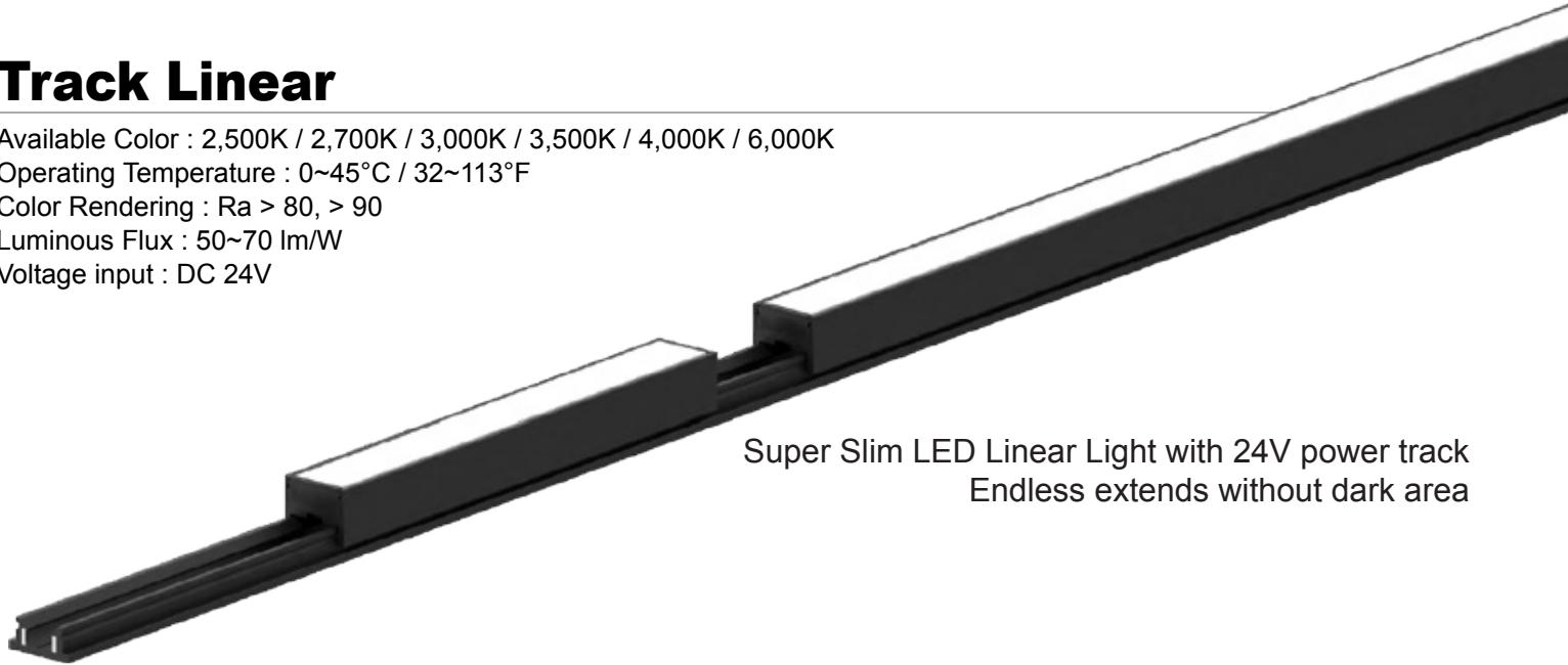
Track Linear
